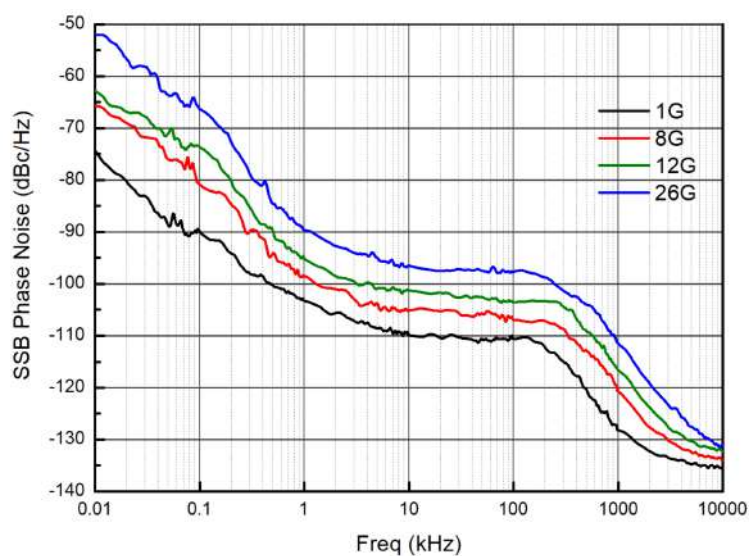
SSB Phase Noise
